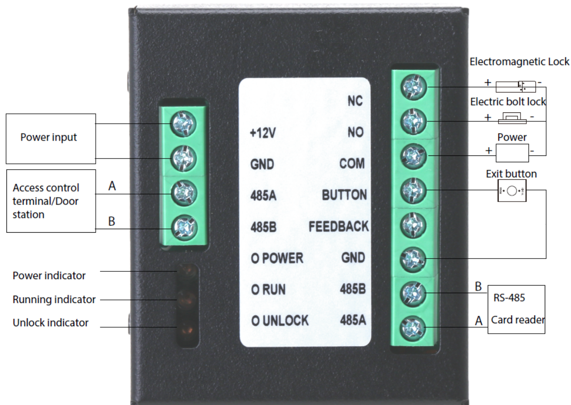
Figure 3-1 Ports description
